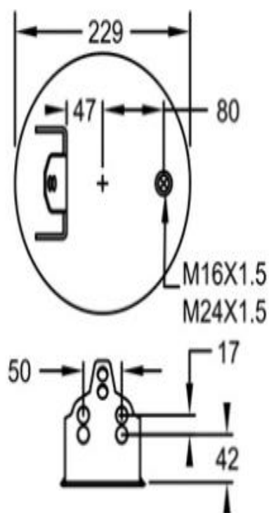
2873 BEAD PLATE
