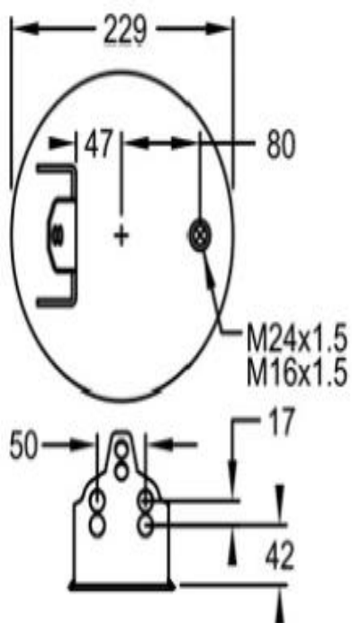
2837 BEAD PLATE
